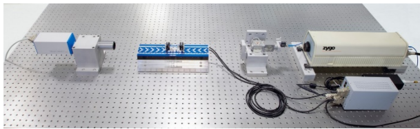
Fig. 2 A typical measurement setup, from left: an autocollimator to measure angular errors, a positioning axis on which two reflecting mirrors are mounted, and an interferometer setup to measure the displacement.
